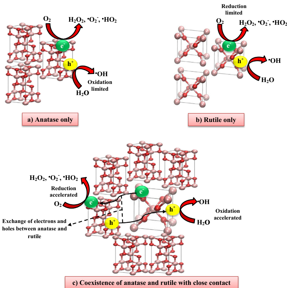
Fig. 3. Possible mechanism for enhancement of photocatalytic disinfection of viruses caused by contacting between anatase and rutile phases of TiO 2 (The modified illustration with permission from reference [67] 2006 Elsevier).
