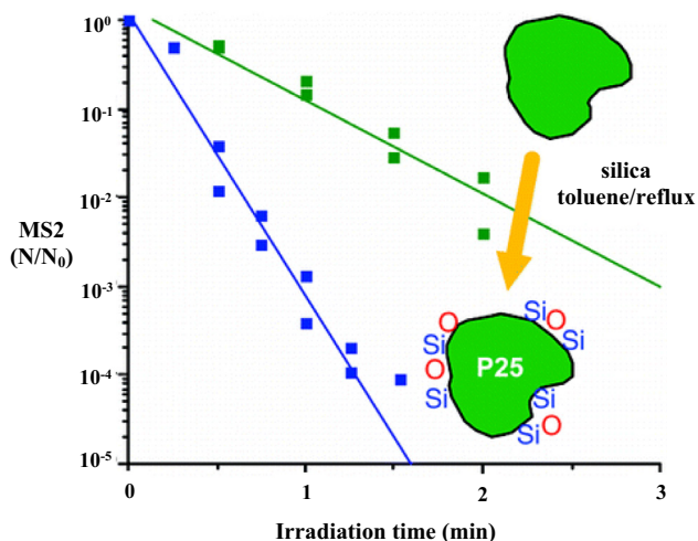
Fig. 4. Photocatalytic inactivation of MS2 by TiO 2 (P25) (green, R 2 = 0.935), and TiO 2 (P25)-SiO 2 (blue, R 2 = 0.970) photocatalysts (Reproduced with permission from reference [71] Copyright 2011 Elsevier). (For interpretation of the references to colour in this figure legend, the reader is referred to the web version of this article.)
